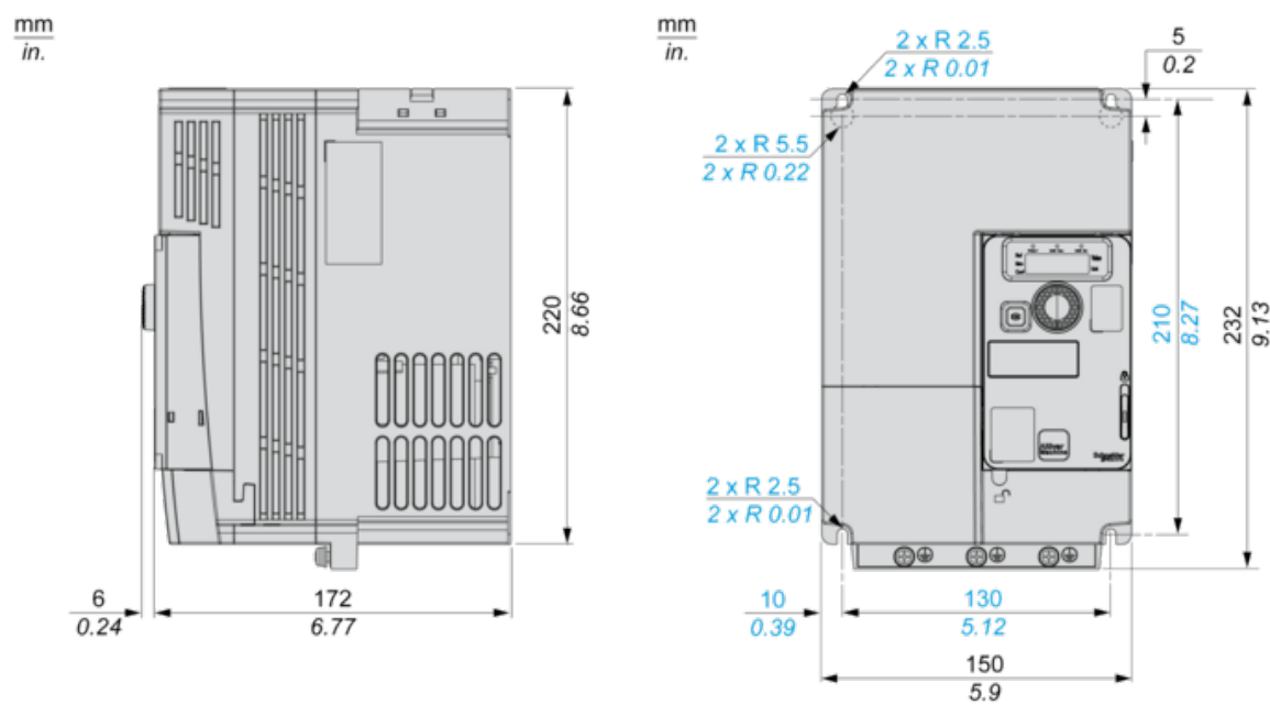
Right and Front Views with EMC Plate
