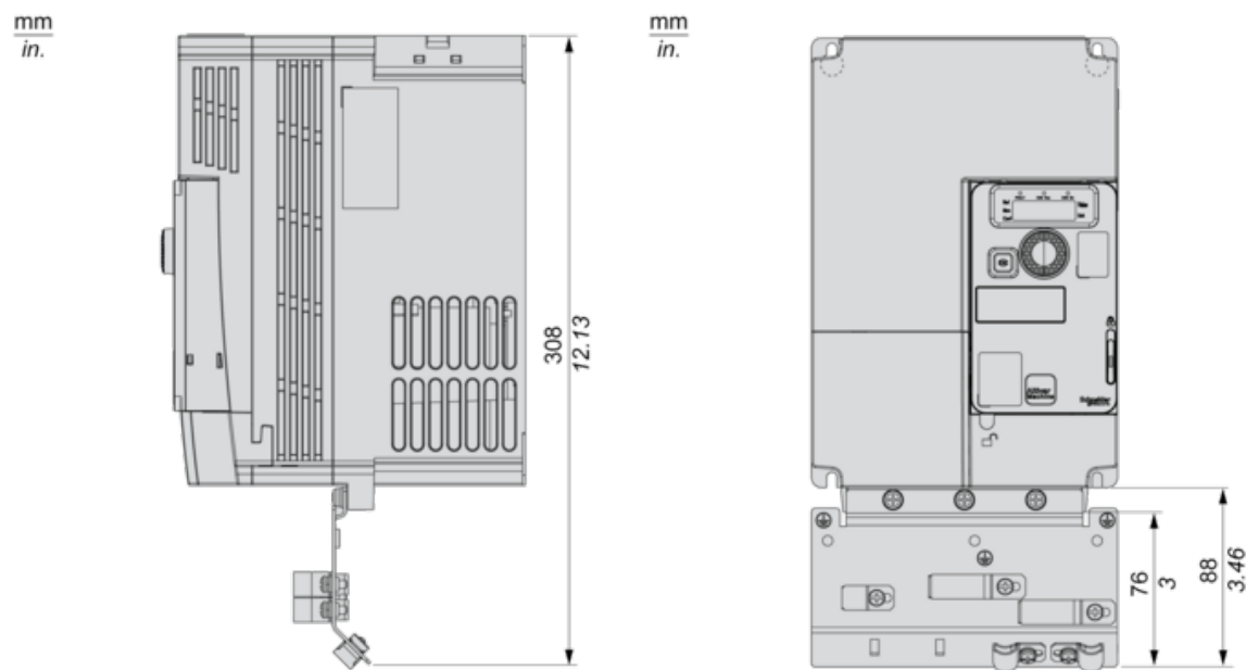
Right and Front Views with EMC Plate
